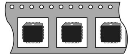
Typical PLCC Package Orientation Package Code (FN)
