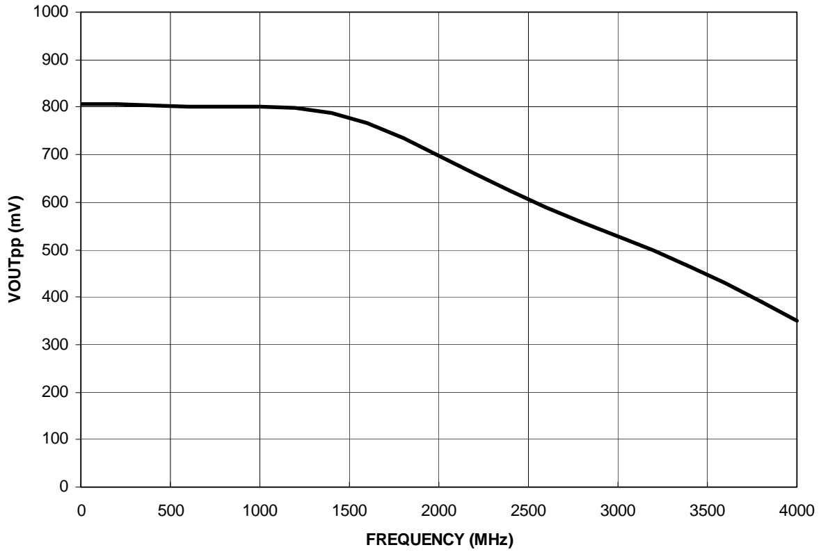
Fig 1: Typical Large Signal Outputs, Q HG /Q HG
